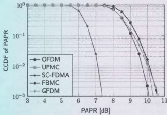
Fig.2: CCDF of PAPR
