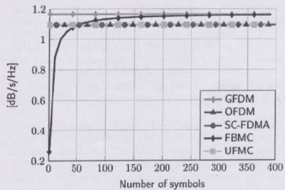
Fig.1: Spectral Efficiency versus number of symbols
